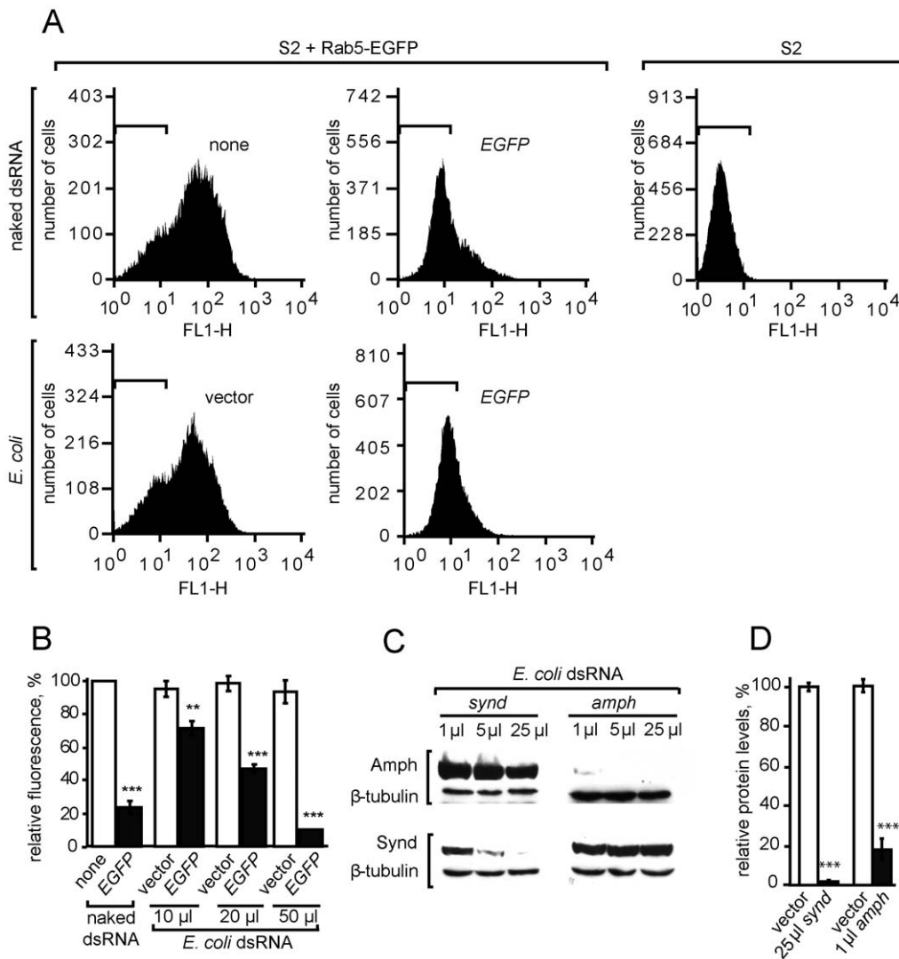
Figure 2. Efficiency and specificity of RNAi induced by dsRNA-expressing E. coli . (A) Fluorescence loss in Rab5-EGFP-expressing S2 stable cell line due to RNAi induced either by 1 μg of naked EGFP dsRNA or by 50 μl of EGFP dsRNA-expressing E. coli . Representative FACS histograms are showing numbers of S2 cells with different fluorescence intensities. Horizontal bars in each graph (approximately 100 to 101) show the fluorescence range of wild-type S2 cells (as in the top right histogram). (B) Quantification of EGFP fluorescence levels in Rab5-EGFP-expressing S2 cells, treated with either 1 μg of EGFP dsRNA or varying quantities of E. coli (OD 600 =1.2) that express EGFP dsRNA. The graph shows the level of EGFP fluorescence, normalized to cells treated with no RNAi. (C) Western blots of amphiphysin, syndapin or β-tubulin in lysates from S2 cells treated for 72 hours with E. coli that express amph or synd dsRNA. (D) Bar graph shows levels of amphiphysin and syndapin relative to β-tubulin. Knockdown was quantified in S2 cells treated with E. coli that expressed synd (25 μl) or amph (1 μl) dsRNA; amphiphysin was undetectable after treatment with larger amounts of E. coli . Values are averages of three independent experiments. Error bars indicate standard error of the mean. ** P<0.01; *** P<0.005; two-tailed t-test.
