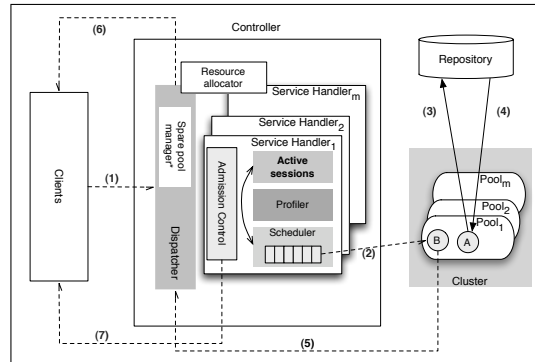
Fig. 2. Architecture overview. Dotted lines indicate asynchronous messages.
