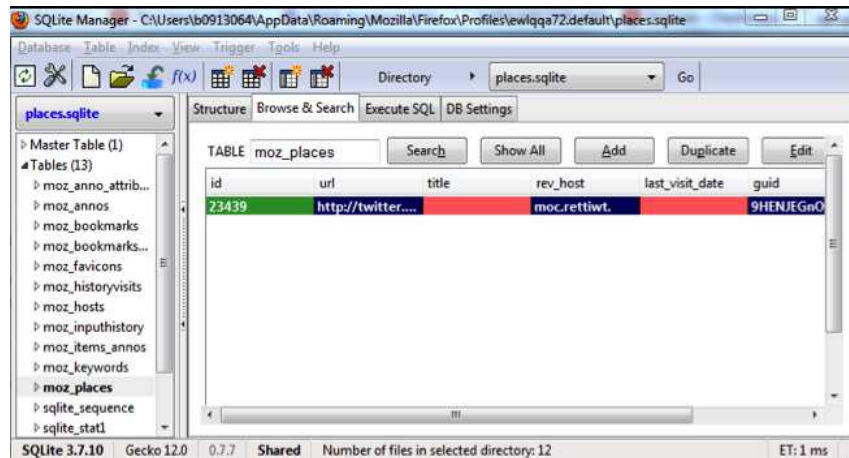
(b) Record in moz_places with deleted last_visit_date
