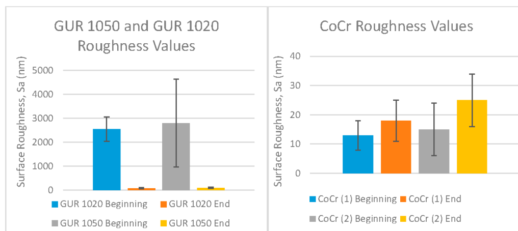
Figure 4. Change in roughness of the materials used. (left) Ultra High Molecular Weight Polyethylene (UHMWPE pins), (right) CoCr discs.
