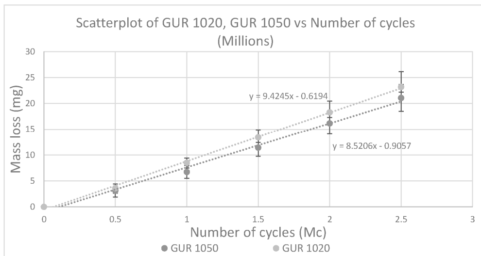
Figure 1. Comparative mean wear rate of GUR 1020 and GUR 1050 with the first 500,000 cycles.
