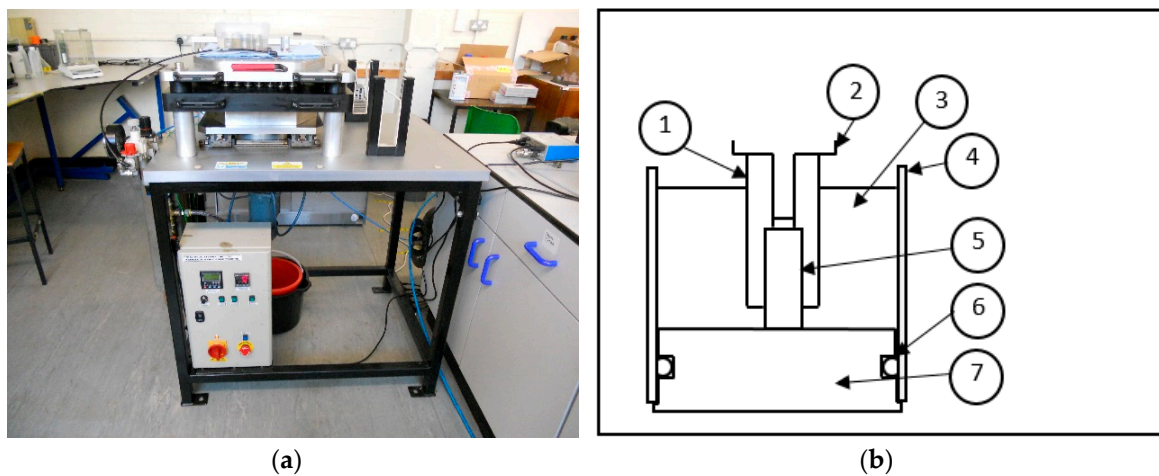
Figure 5. (a) General view of the SuperCTPOD; (b) Pin-on-Disc schematic (1) Polyacetal Pin Holder (2) Load application module (3) Lubricant (4) Lubricant container (5) Pin sample (6) Silicone O-ring (7) Disc sample.
