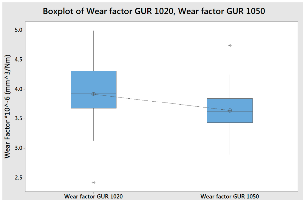
Figure 3. Box plot of the wear factors of GUR 1020 and GUR 1050 with mean values of 3.92 \times 10^{-6} \text{ mm}^3/\text{Nm} and 3.64 \times 10^{-6} \text{ mm}^3/\text{Nm} , respectively.
