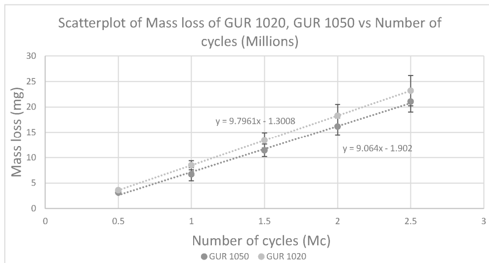
Figure 2. Comparative mean wear rate of GUR 1020 and GUR 1050 without the first 500,000 cycles.
