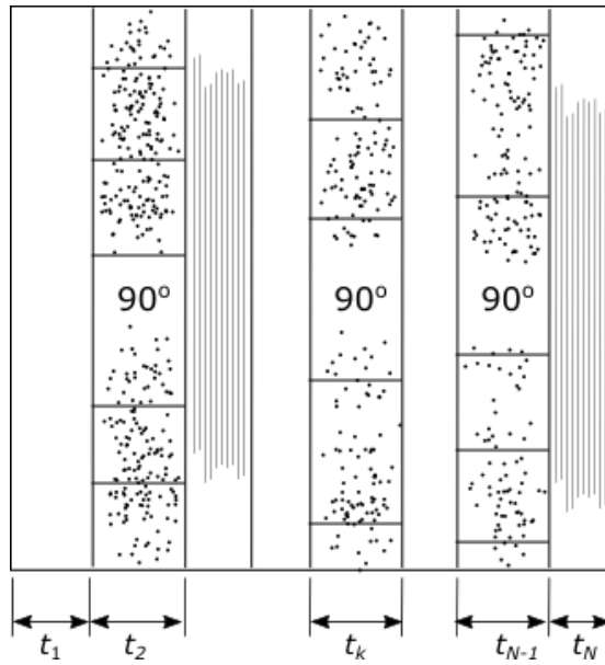
Figure 1: Schematic presentation of a cracked laminate in the rotated coordinate system.
