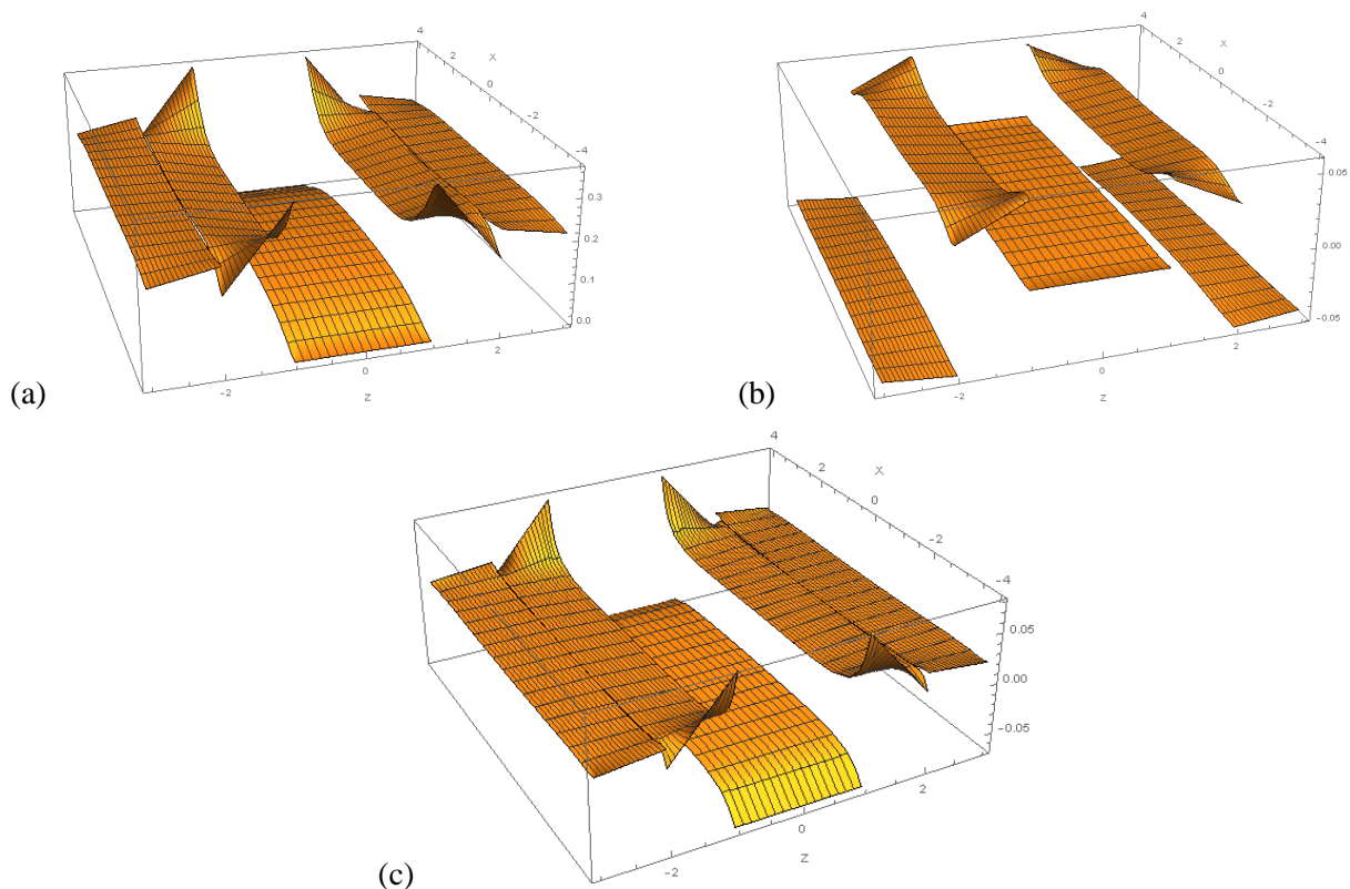
Figure 3: Stress distribution in [\pm 15/90]_s : (a) \sigma_{xx} , (b) \sigma_{xy} , (c) \sigma_{yy}
