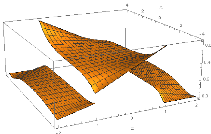
Figure 4: Distribution of \sigma_{xx} in [90/0]_s with staggered arrangement of cracks.
