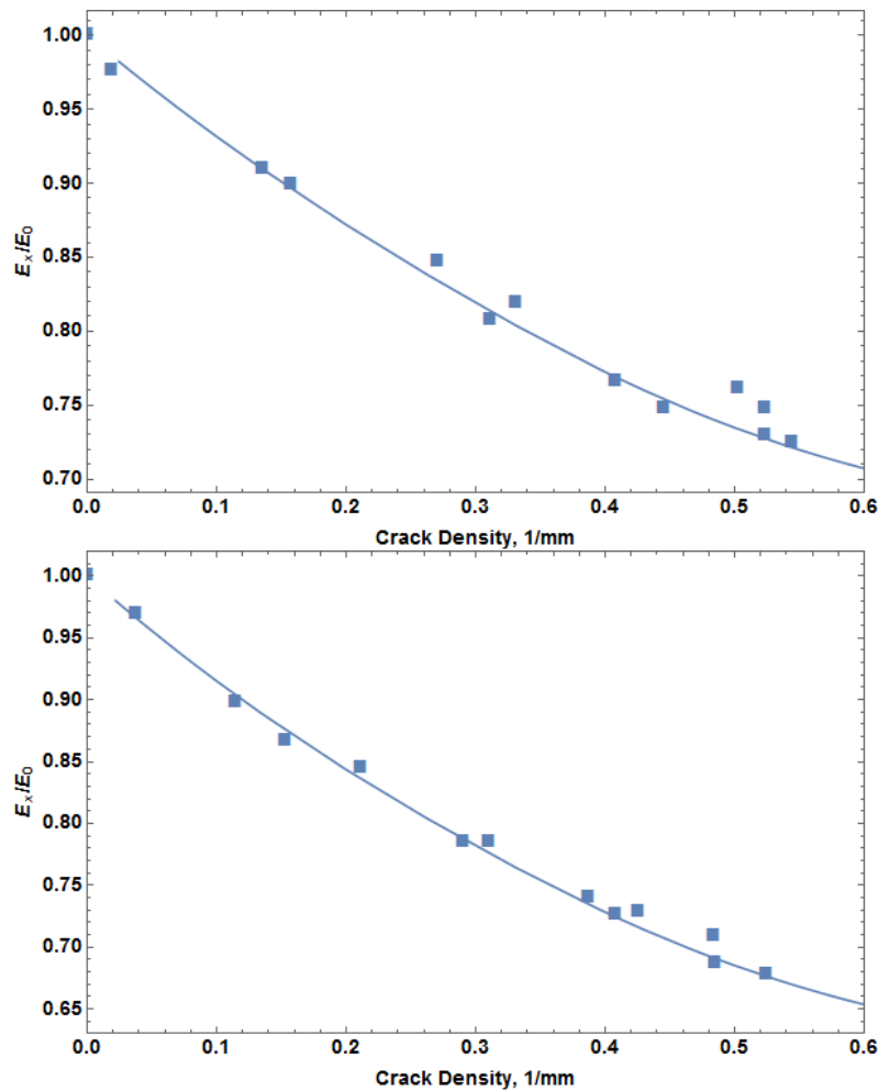
Figure 5: Young modulus reduction as a function of transverse crack density in [\pm 15/90_4]_s (top) and [\pm 30/90_4]_s (bottom). Experimental data from [8].
