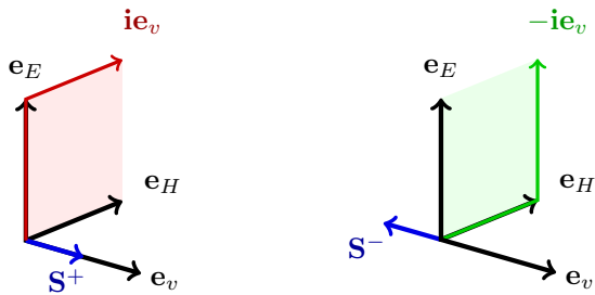
FIG. 1. Schematic of electron spin and field vectors ( \mathbf{S} , \mathbf{e}_E , and \mathbf{e}_H , respectively) and the vector of motion, \mathbf{e}_v , for an electron, with both the parallel (left) and antiparallel (right) behaviour. The direction of the electron spin vector, \mathbf{S}^\pm , is shown by the short arrows on the \mathbf{e}_v axis in both cases.
