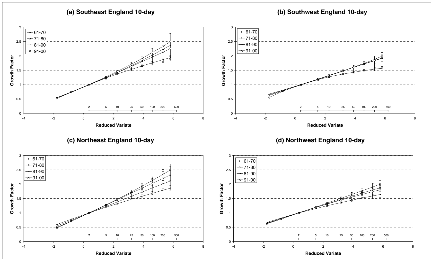
Figure 7. Decadal change in the 10-day growth curve: (a) SEE; (b) SWE; (c) NEE; (d) NWE.
