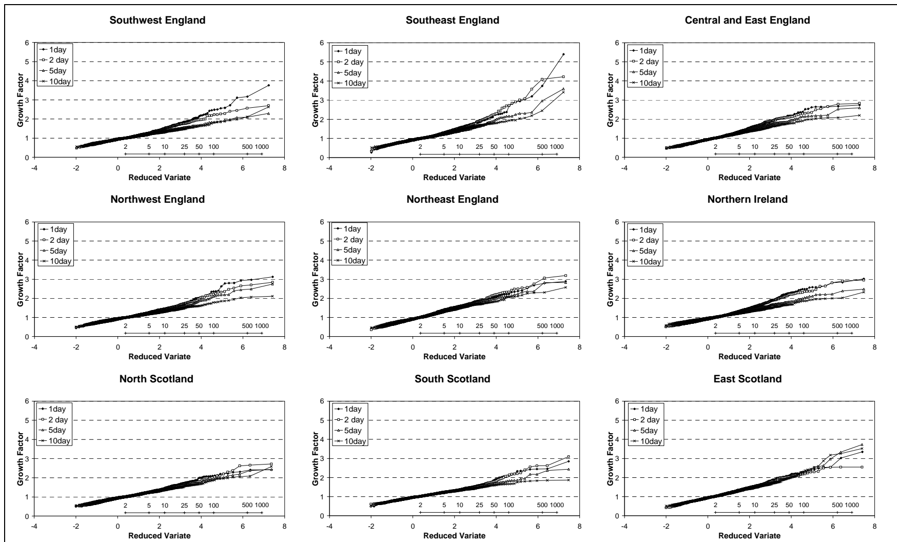
Figure 3. Shape of standardized annual maximum distributions for the nine pooling regions.
