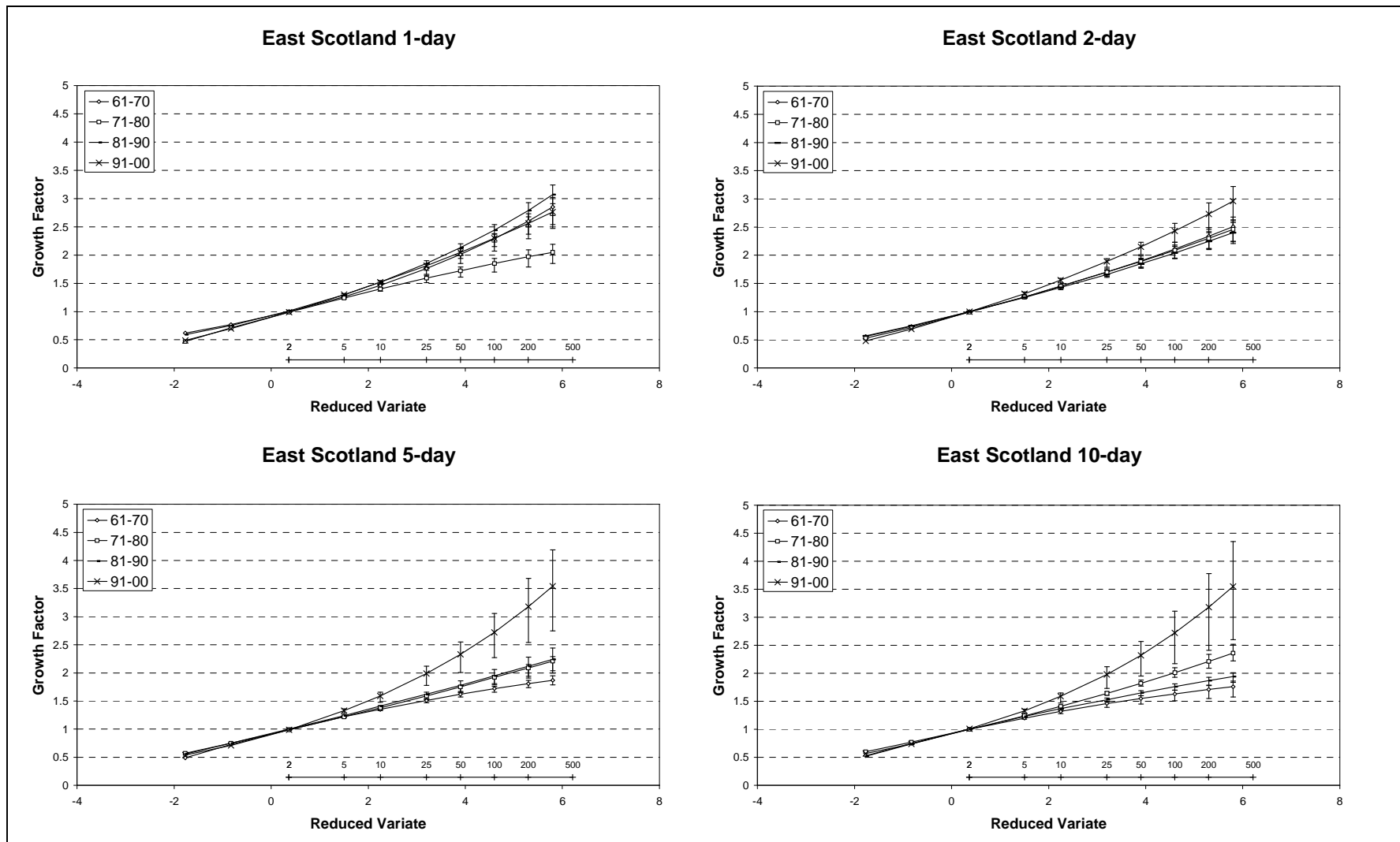
Figure 8. Decadal change in the 1-, 2-, 5- and 10-day growth curves in the ES pooling region.
