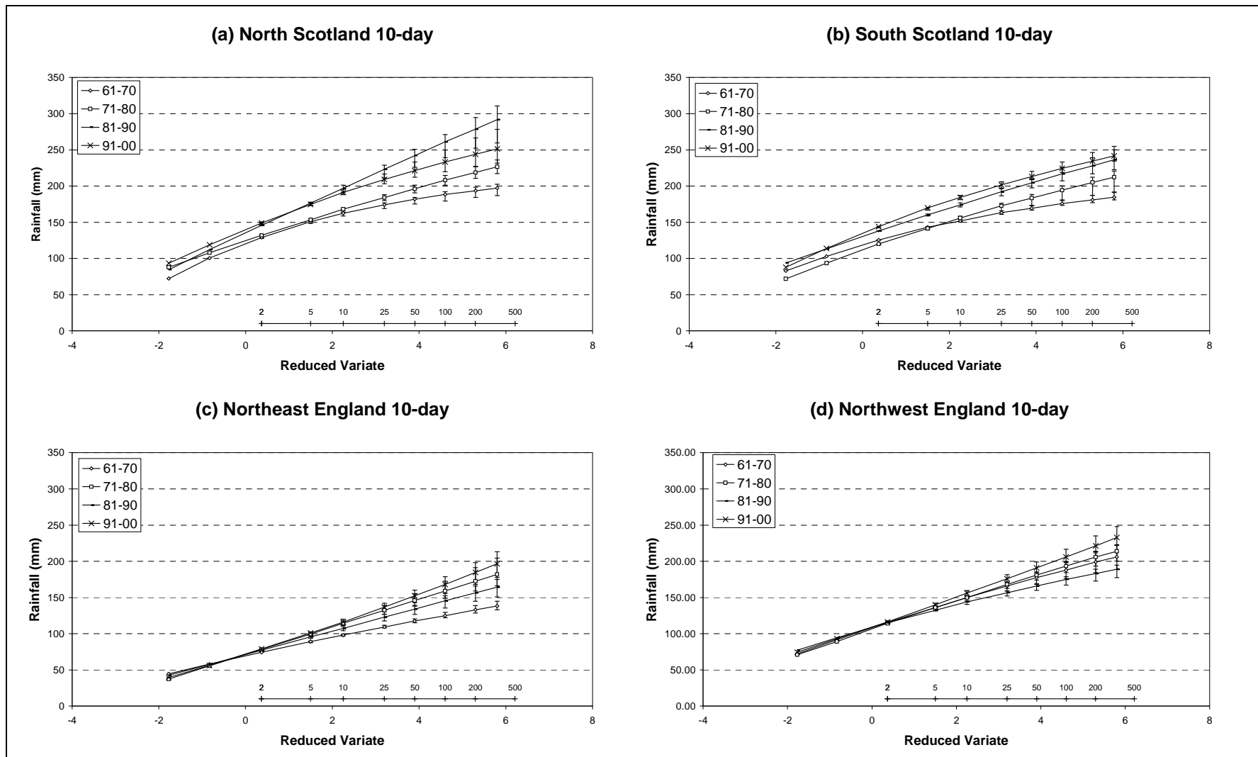
Figure 11. Decadal changes in 10-day duration return period estimates using mean regional RMED for: (a) NS; (b) SS; (c) NEE; (d) NWE.
