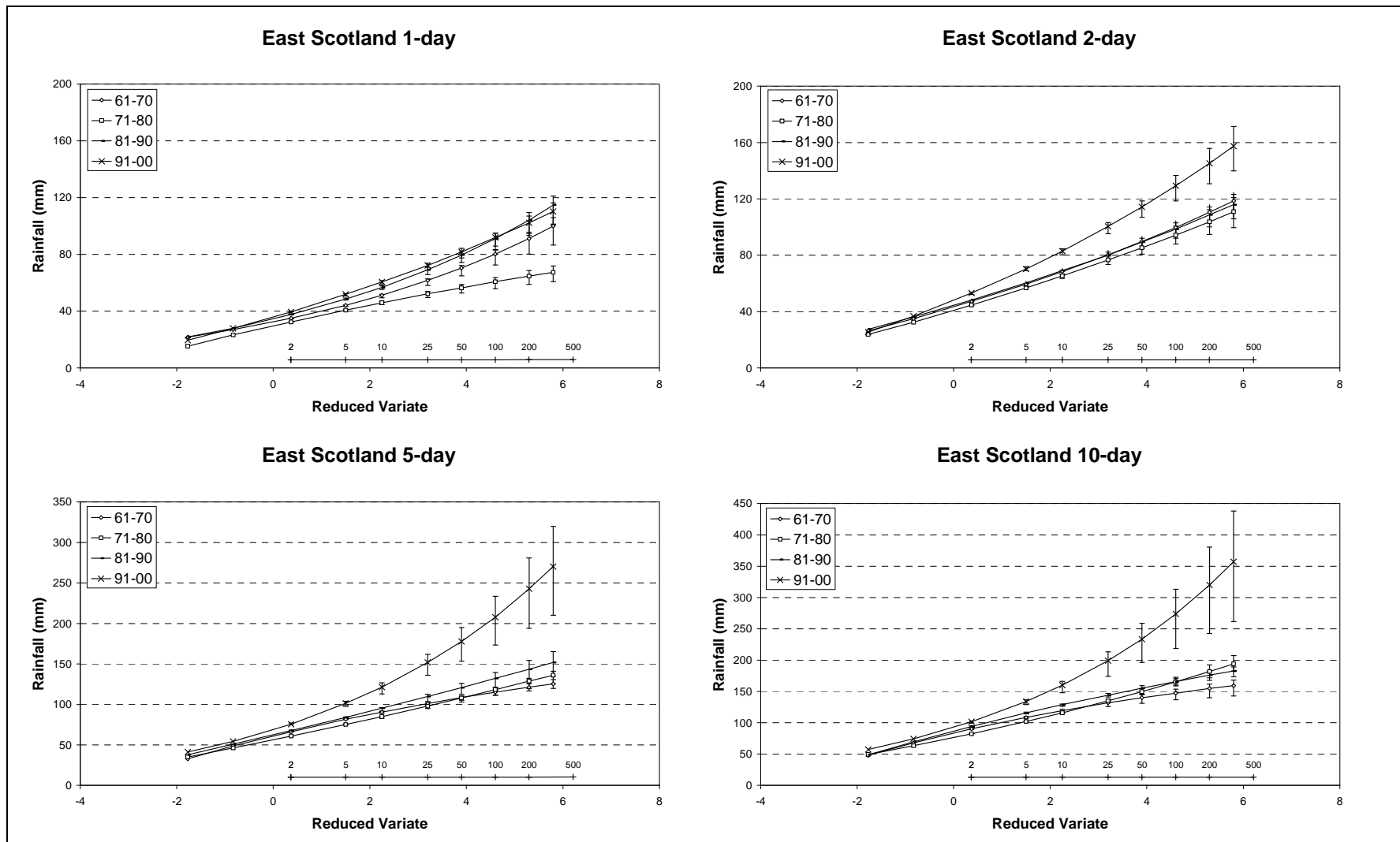
Figure 10. Decadal changes in return period estimates using mean regional RMED for the ES pooling region.
