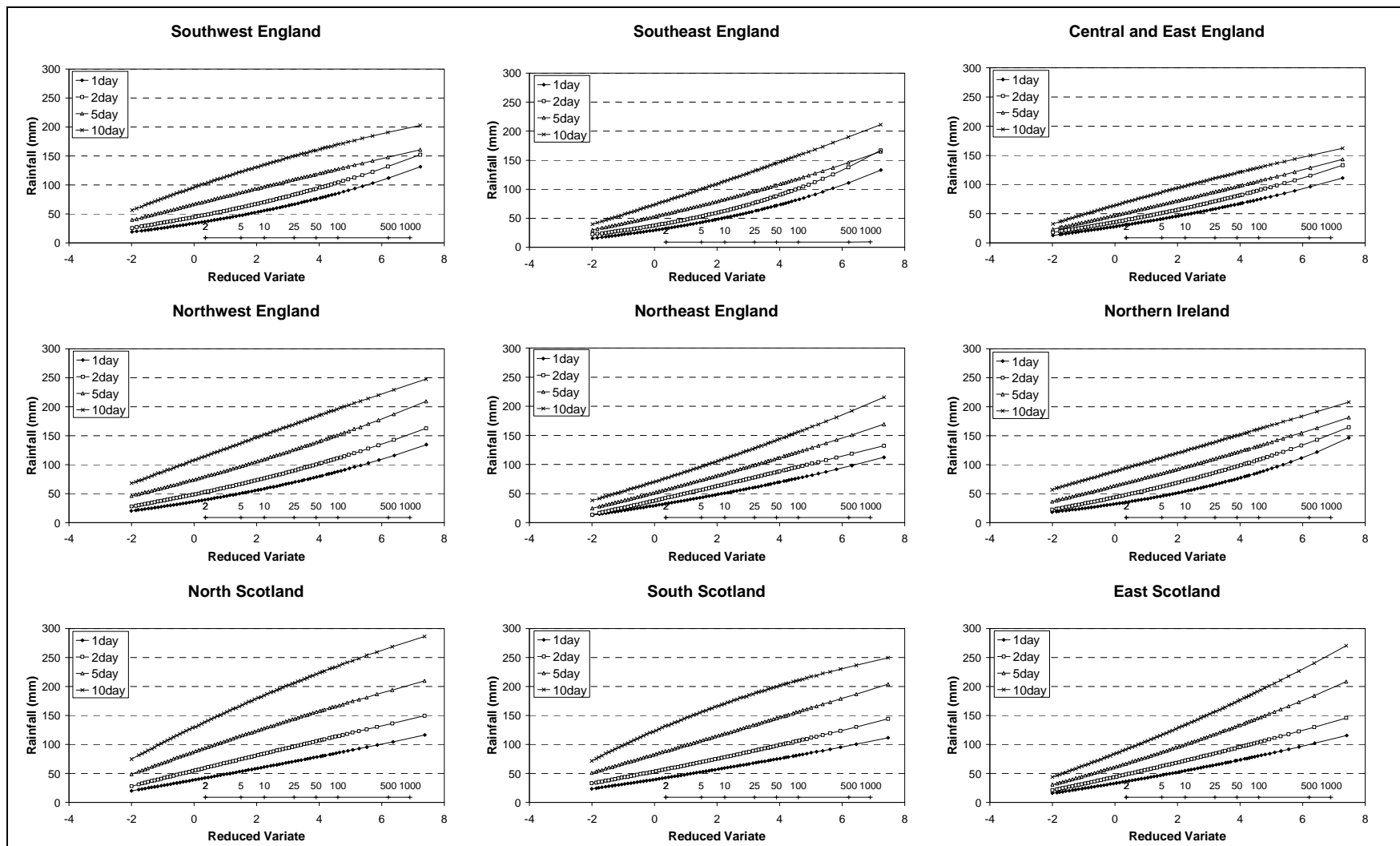
Figure 5. Fitted annual maximum GEV distributions for the nine pooling regions (using mean regional RMED from 1961-1990 as a multiplier).
