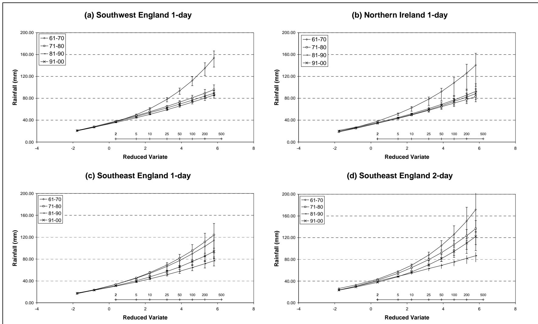
Figure 9. Decadal change in RMED: (a) SWE 1-day; (b) NI 1-day; (c) SEE 1-day; (d) SEE 2-day.
