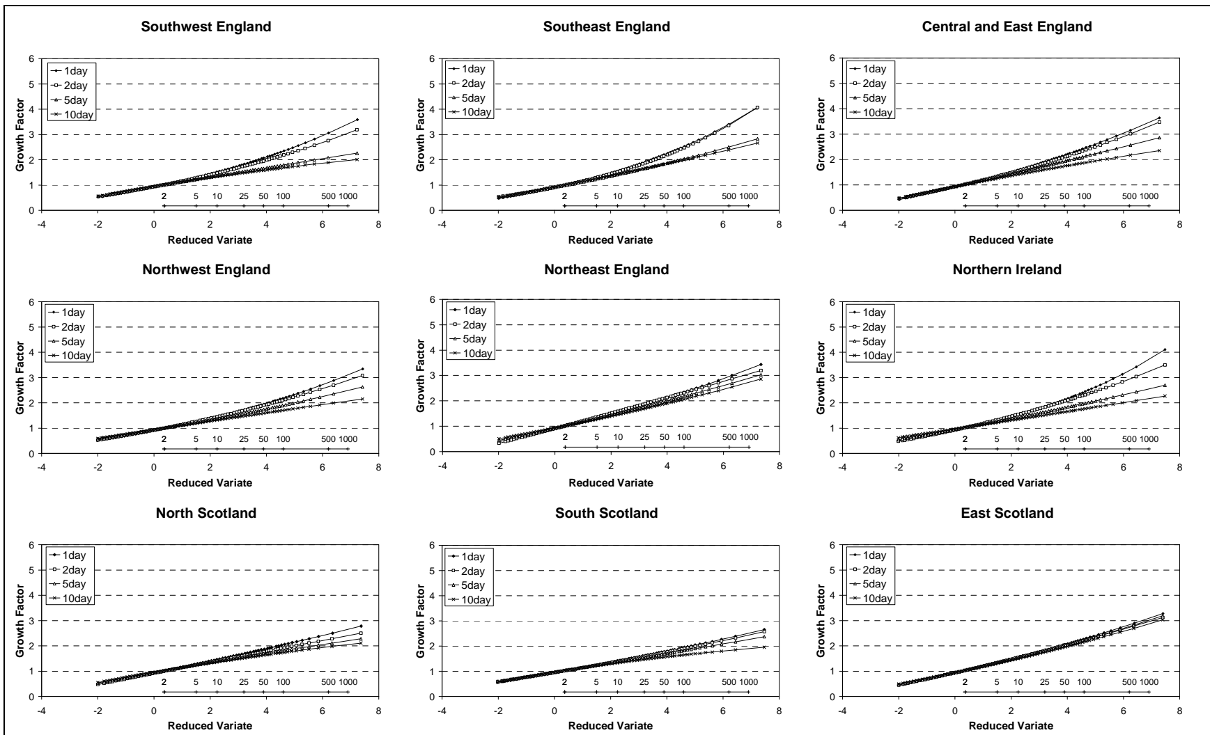
Figure 4. Fitted standardized annual maximum GEV distributions for the 9 regions.
