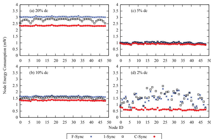
Figure 14: Individual node energy consumptions in 7x7 grid networks with 40 ppm drift rate at different duty-cycles
