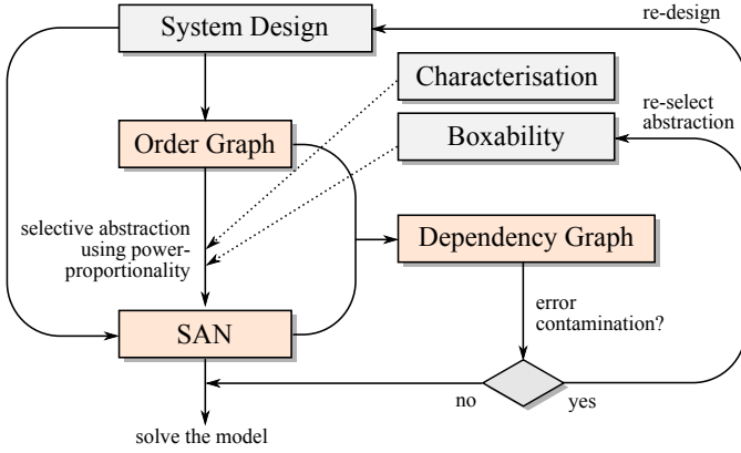
Figure 2. The flowchart of the proposed method.
