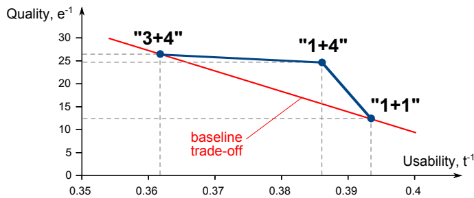
Figure 10. Simulation results in the Quality/Usability trade-off diagram
