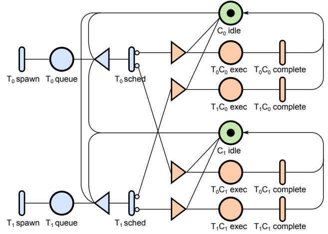
Figure 6. Model for the naïve scenario leading to error contamination.
