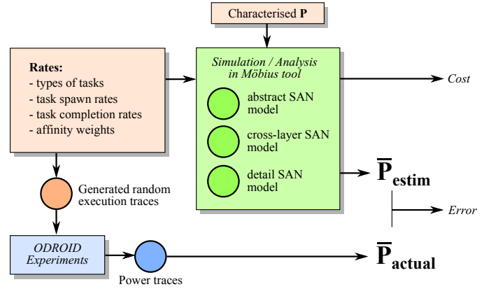
Figure 5. Model evaluation framework.
