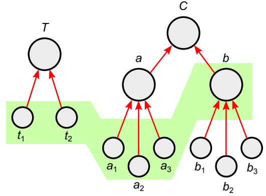
Figure 3. Example vertical view of an Order Graph with a cross-layer cut.
