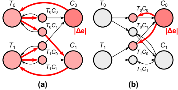
Figure 9. Dependency graphs with highlighted error contamination paths: (a) for Figure 6, (b) for Figure 7.
