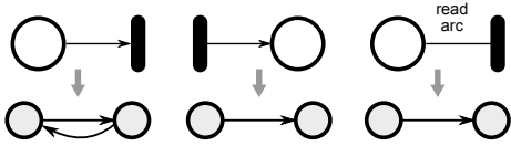
Figure 8. Rules for SAN mapping to dependency graphs.
