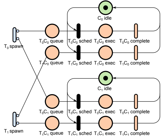
Figure 7. Fixed affinities in the scenario produce a better model.
