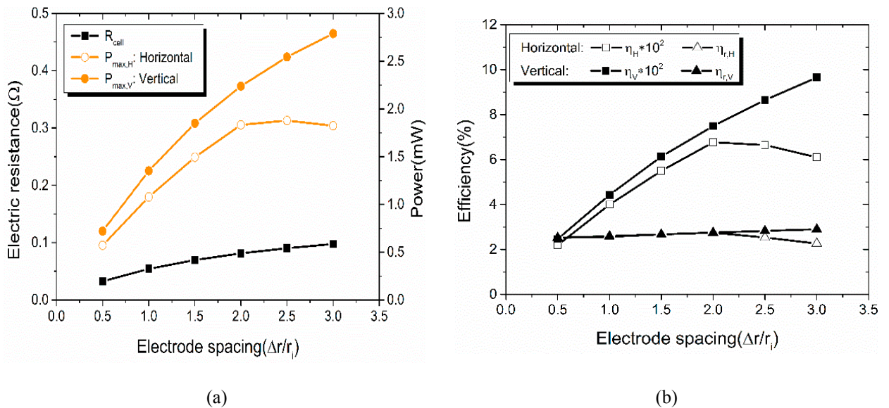
Fig. 4. (a) Diagram of electric resistance and power; (b) Diagram of efficiency and relative efficiency
