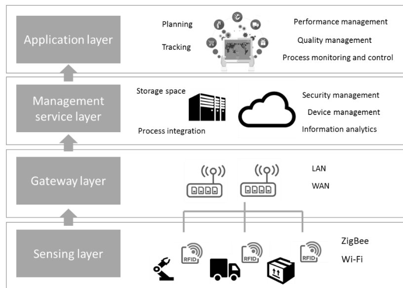
Figure 2. Supply chain IoT architecture
