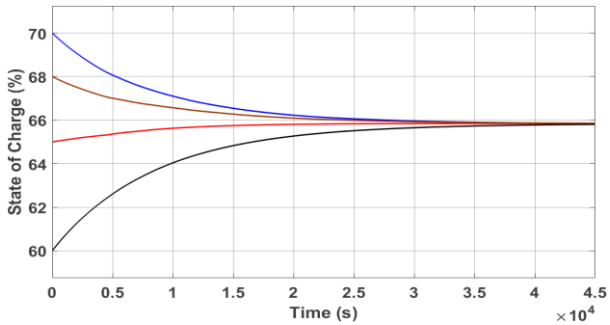
Figure 9. The cell SoCs with optimized SC
