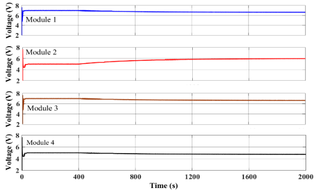
Figure 12. The voltage of each module at the series connected side with 0.2C battery current
