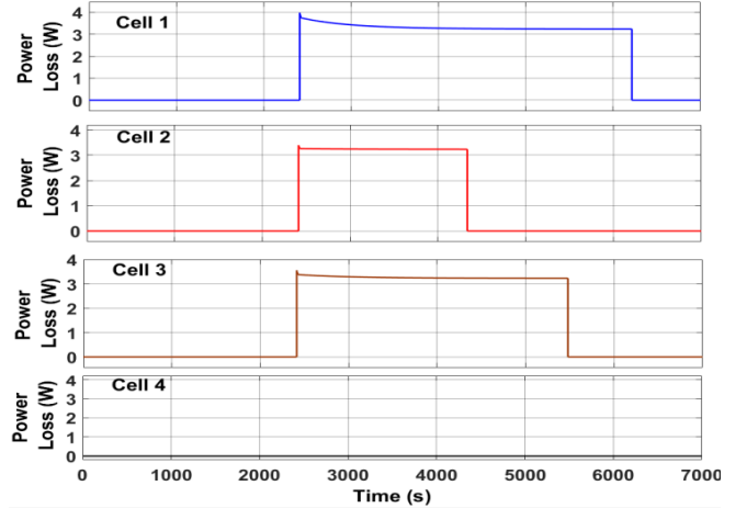
Figure 7. Power losses with switched shunt resistor method, 1A balancing current
