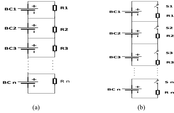
Figure 1. Dissipative Cell Balancing Circuits: a) Fixed Shunt Resistor, b) Switched Shunt Resistor
