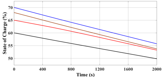
Figure 13. Convergence of cell SoCs with 0.2C battery load
