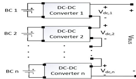
Figure 3. Runtime Cell Balancing Structure
