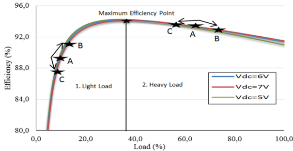
Figure 14. Typical converter efficiency curve
