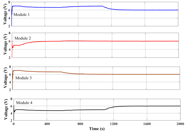
Figure 10. The voltage of each module at the series connected side with 0.8C battery load
