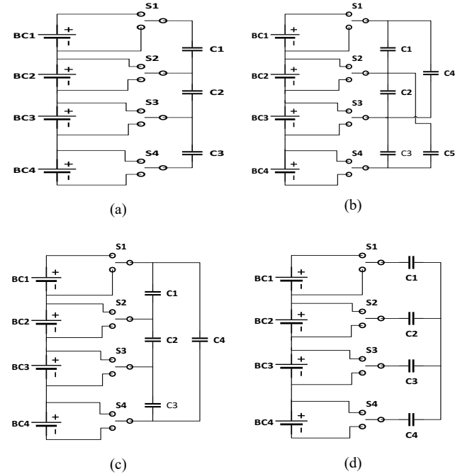
Figure 2. Capacitor Cell Balancing Circuits: a) Switched Capacitor (SC), b) Double Tiered SC, c) Chain Structure SC, d) Optimized SC
