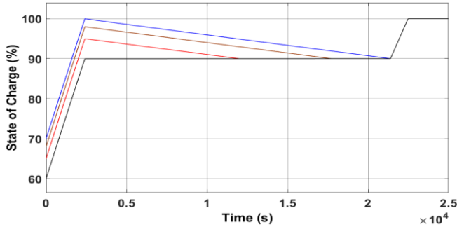
Figure 4. The cell SOC's with switched shunt resistor method, 200mA balancing current
