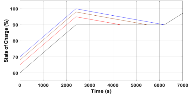
Figure 6. The cell SOC's with switched shunt resistor method, 1A balancing current
