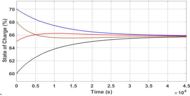
Figure 8. The cell SoCs with SC
