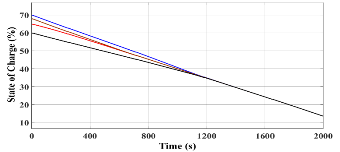
Figure 11. Convergence of cells SoC with 0.8C battery load
