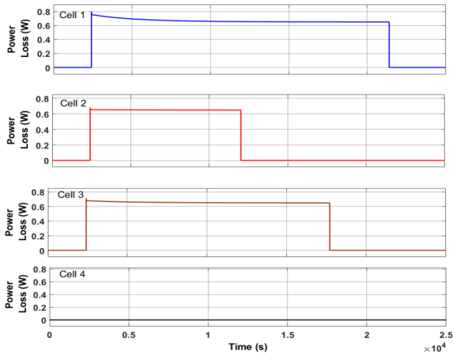
Figure 5. Power losses with switched shunt resistor method, 200mA balancing current
