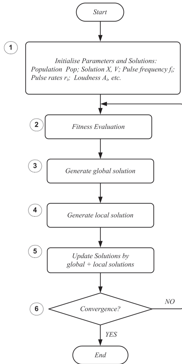
Fig. 3. BAVP flowchar.
