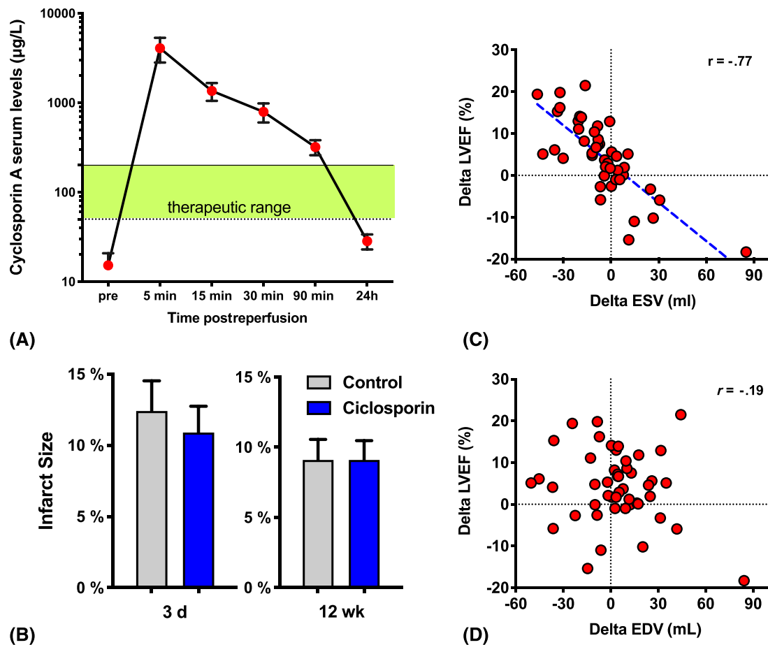
FIGURE 2 Cyclosporin does not affect cardiac remodelling post infarction. (A) Cyclosporin serum level kinetics for n = 8 randomly selected patients from cyclosporin group (displayed as mean \pm standard error of the mean per time point). (B) Infarct size after 3 days and 12 weeks. (C, D) correlation of changes in left ventricular ejection fraction (LVEF), end-diastolic volume (EDV) and end-systolic volume (ESV) in 48 patients with both magnetic resonance images (Spearman r )
