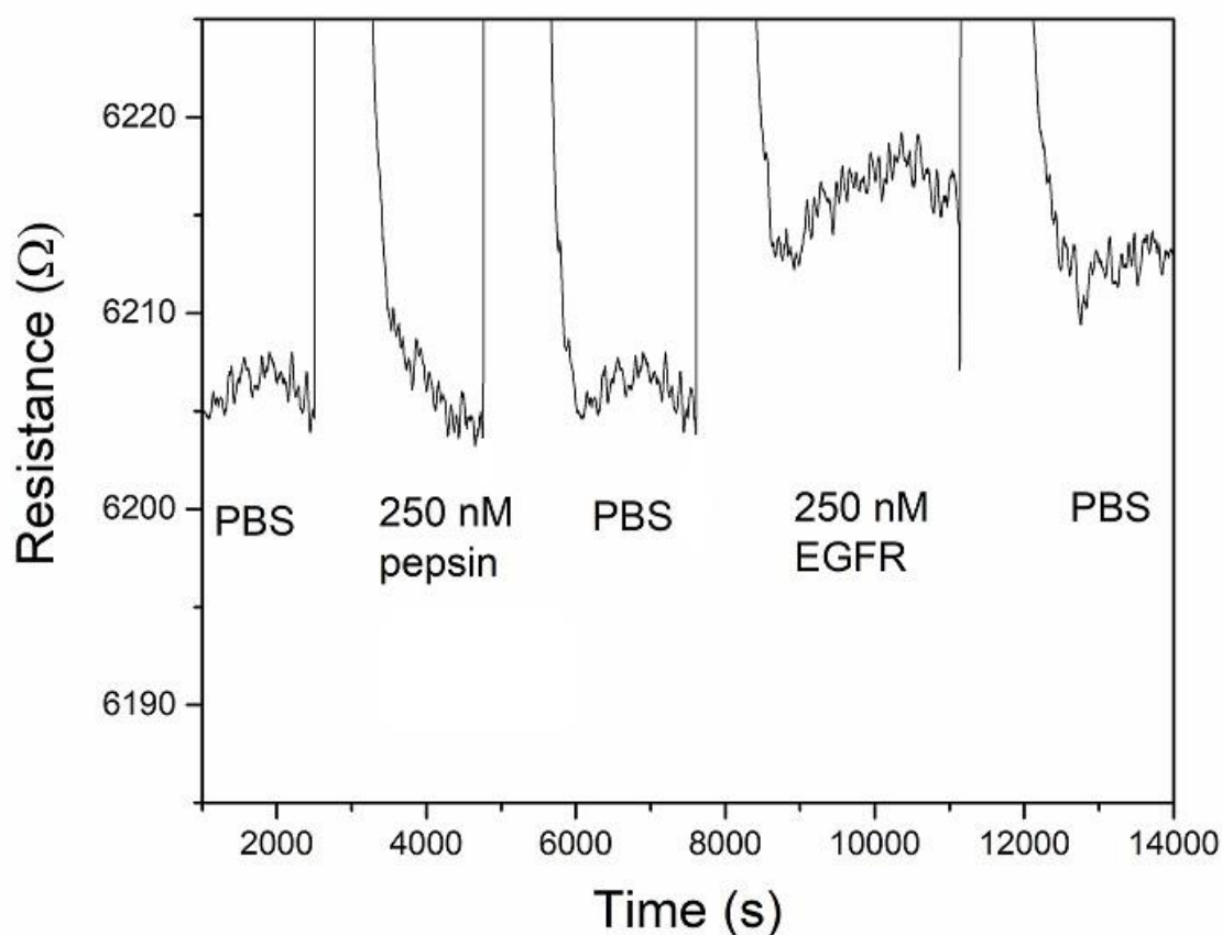
Figure 4. The electrical resistance measured by the thermistor functionalised with a nanoMIP for EGFR upon exposure to pepsin, PBS, and the template EGFR
