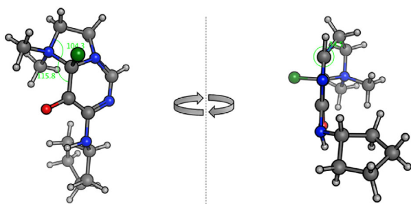
FIGURE 1 Energy minimized intermediate for the S_NAr cyclization leading to 9
