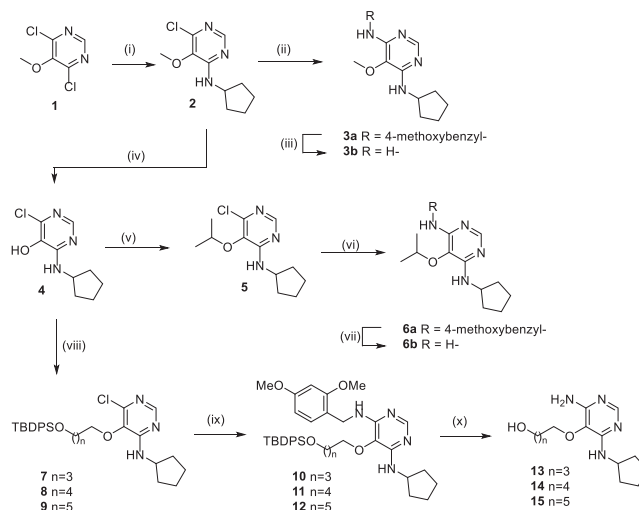
SCHEME 1 Reagents and conditions. (i) Cyclopentylamine, toluene, reflux, 93%; (ii) p -methoxybenzylamine, DIPEA, dioxane, 220 °C, MW, 58%; (iii) TFA, DCM, reflux, 50%; (iv) BBr_3 , DCM, reflux, 98%; (v) 2-bromopropane, K_2CO_3 , MeCN / DMF, 80 °C, 95%; (vi) p -methoxybenzylamine, DIPEA, dioxane, 220 °C, MW, 50%; (vii) TFA, DCM, reflux, 67%; (viii) RX, K_2CO_3 , MeCN, DMF, 80 °C, n = 3 (RX = TBDPSO[CH 2 ] 4 Cl), 73%, n = 4 (RX = TBDPSO [CH 2 ] 5 Cl), 28%, n = 5 (RX = TBDPSO[CH 2 ] 5 Br), 27%; (ix) 2,4-dimethoxybenzylamine, DIPEA, dioxane, 220 °C, MW, n = 3 , 33%, n = 4 , 41%, n = 5 , 54%; (x) TFA, DCM, reflux, n = 3 , 38%, n = 4 , 55%, n = 5 , 61%
