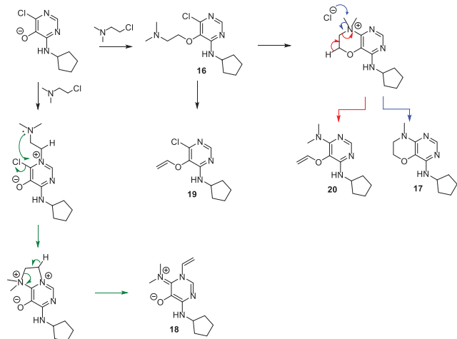
SCHEME 3 Proposed mechanism of formation of 17 , 18 , 19 , and 20
