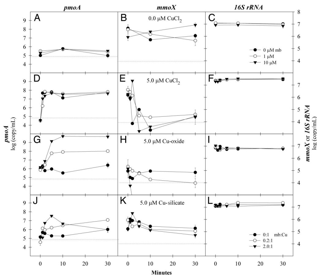
Fig. 1. pmoA (pMMO subunit), mmoX (sMMO subunit), and 16S-rRNA gene transcript levels in a M. trichosporium OB3b presented with different sudden copper exposures: copper-free NSM media (A–C), 5 \mu\text{M} as \text{CuCl}_2 (D–F), 5 \mu\text{M} copper provided as Cu-doped iron oxide (G–I), and 5 \mu\text{M} Cu supplied as Cu-borosilicate glass (J–L). Transcript levels were determined at three different levels of mb: no mb ( \bullet ), 0.2:1 mb:Cu stoichiometry ( \circ ), and 2.0:1 mb:Cu stoichiometry ( \blacktriangledown ). Dashed lines represent RT-PCR detection limits for pmoA and mmoX .
