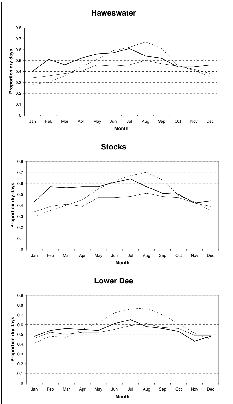
Figure 5 Comparison of catchment proportion dry days for observed data (bold line), bias-corrected HadRM3H control scenario (line) and bias-corrected HadRM3H future scenario (dashed line).
