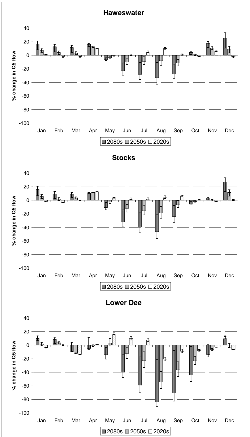
Figure 12 Percentage change in the Q_5 flow between the HadRM3H control and future scenarios for the 2020s, 2050s and 2080s time-slices. Results shown are for the SRES A2 (UKCIP02 Medium-High) emissions scenario, but uncertainty bounds are given for the SRES A1 and B1 (UKCIP02 High and Low) emissions scenarios.
