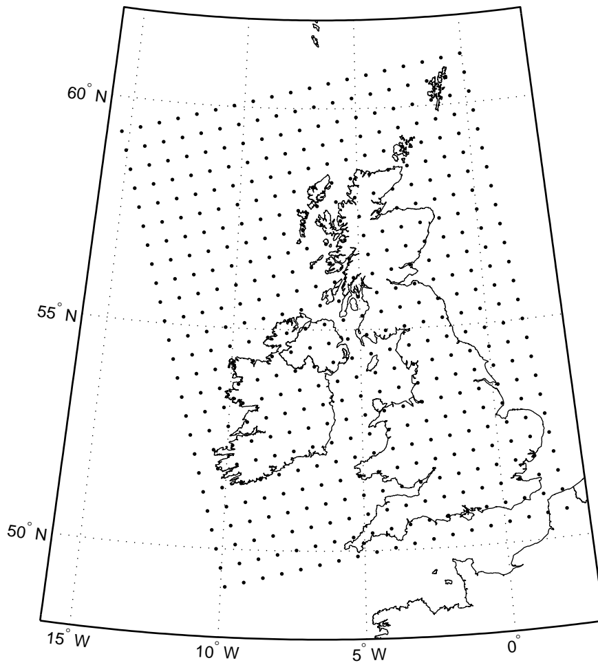
Figure 2 HadRM3H model dataset over the UK where points denote grid box centres (reproduced from Fowler et al. , 2005).
