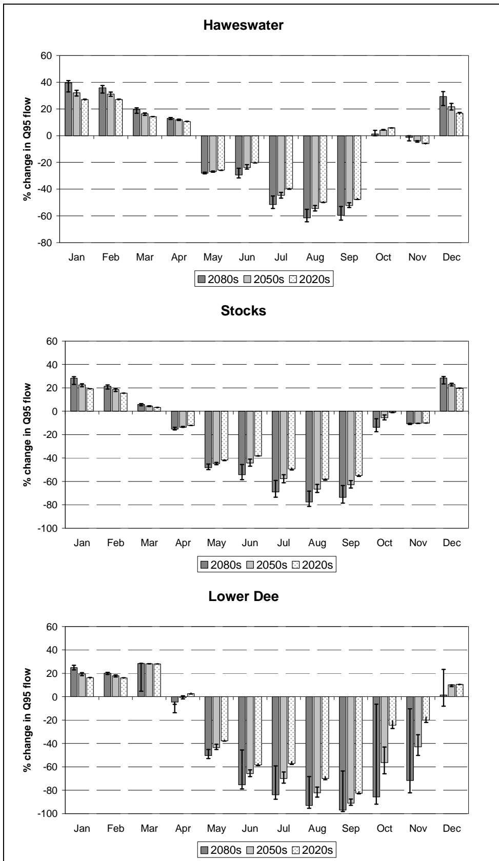
Figure 11 Percentage change in the Q 95 flow between the HadRM3H control and future scenarios for the 2020s, 2050s and 2080s time-slices. Results shown are for the SRES A2 (UKCIP02 Medium-High) emissions scenario, but uncertainty bounds are given for the SRES A1 and B1 (UKCIP02 High and Low) emissions scenarios.
