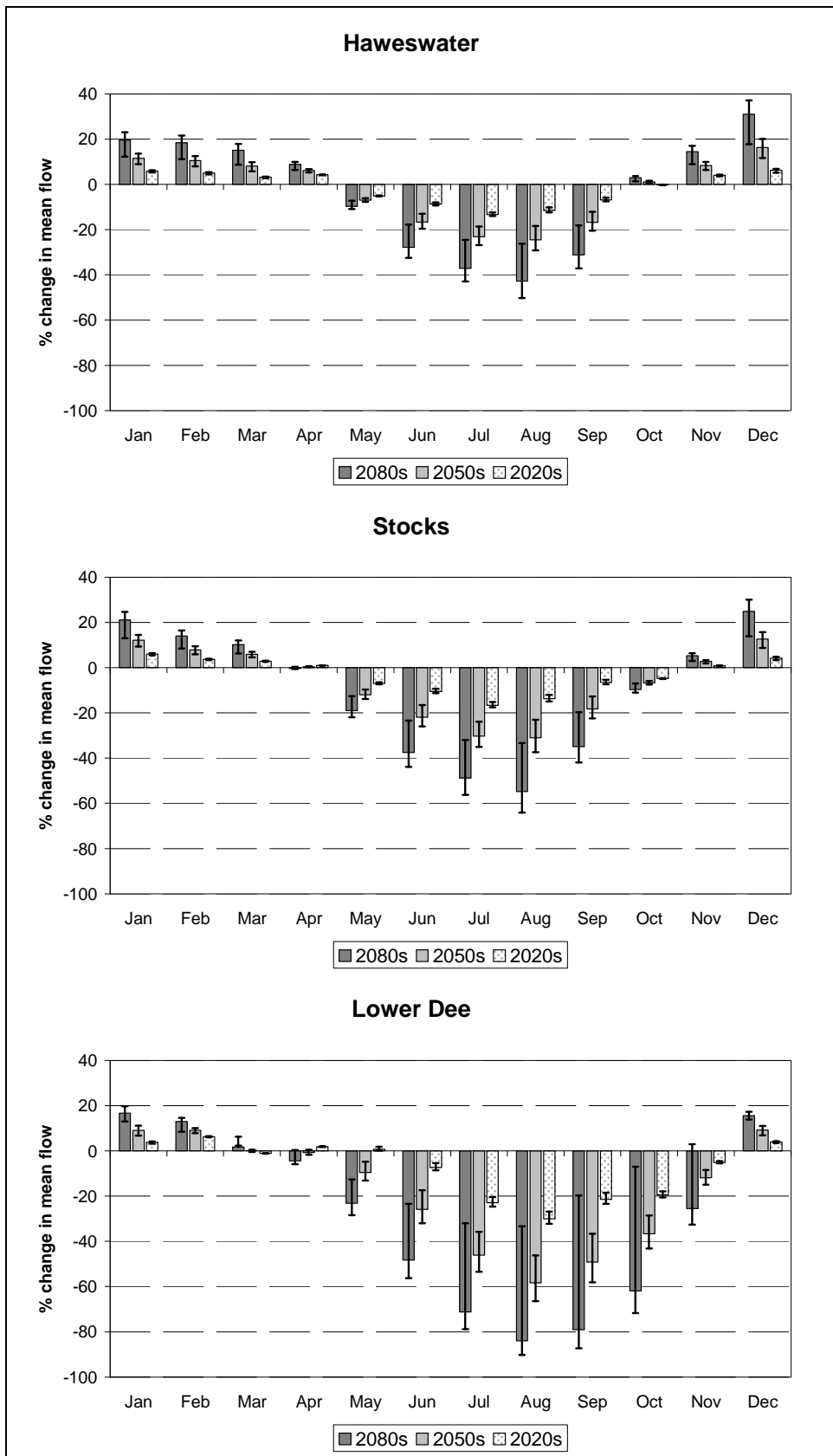
Figure 8 Percentage change in mean monthly streamflow between the HadRM3H control and future scenarios for the 2020s, 2050s and 2080s time-slices. Results shown are for the SRES A2 (UKCIP02 Medium-High) emissions scenario, but uncertainty bounds are given for the SRES A1 and B1 (UKCIP02 High and Low) emissions scenarios.
