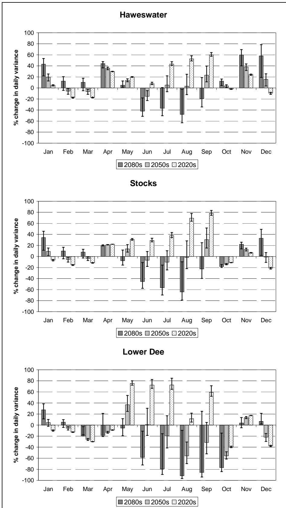
Figure 9 Percentage change in daily streamflow variance between the HadRM3H control and future scenarios for the 2020s, 2050s and 2080s time-slices. Results shown are for the SRES A2 (UKCIP02 Medium-High) emissions scenario, but uncertainty bounds are given for the SRES A1 and B1 (UKCIP02 High and Low) emissions scenarios.
