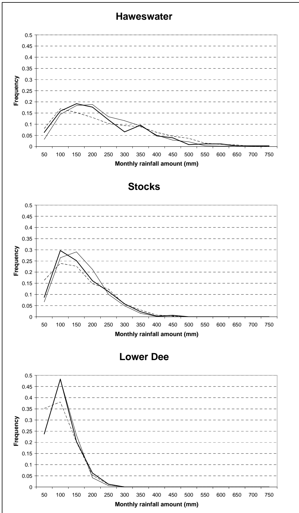
Figure 7 Comparison of distribution of monthly rainfall totals for observed data (bold line), bias-corrected HadRM3H control scenario (line) and bias-corrected HadRM3H future scenario (dashed line).
