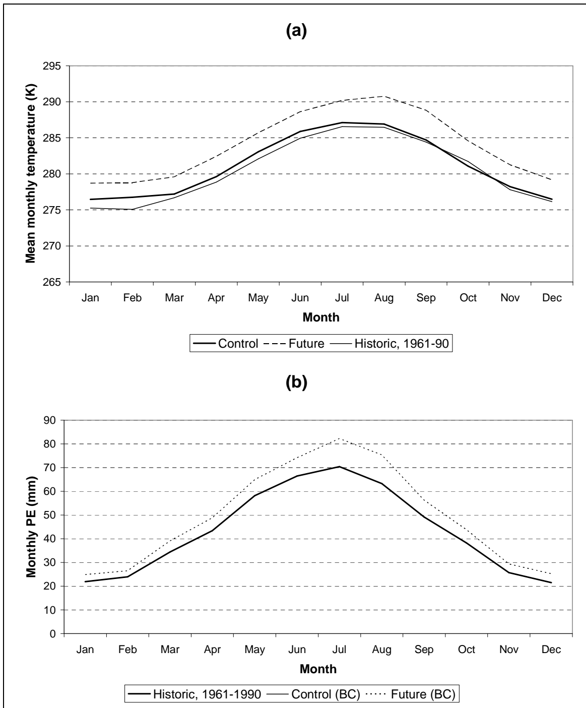
Figure 3 (a) Mean monthly temperature (K), and (b) mean monthly PE, for historic (1961-1990), and HadRM3H control and future scenarios. BC indicates that ‘bias-correction’ of temperature data has been used to match the observed historic series.
