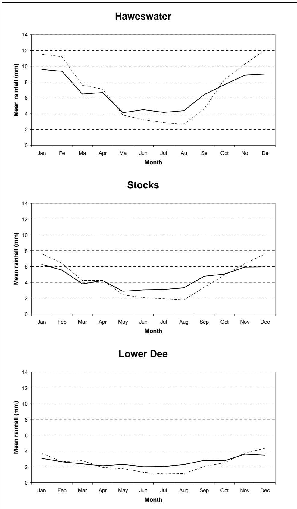
Figure 4 Comparison of catchment monthly mean rainfall (mm) for observed data (bold line), bias-corrected HadRM3H control scenario (bold line) and bias-corrected HadRM3H future scenario (dashed line).
