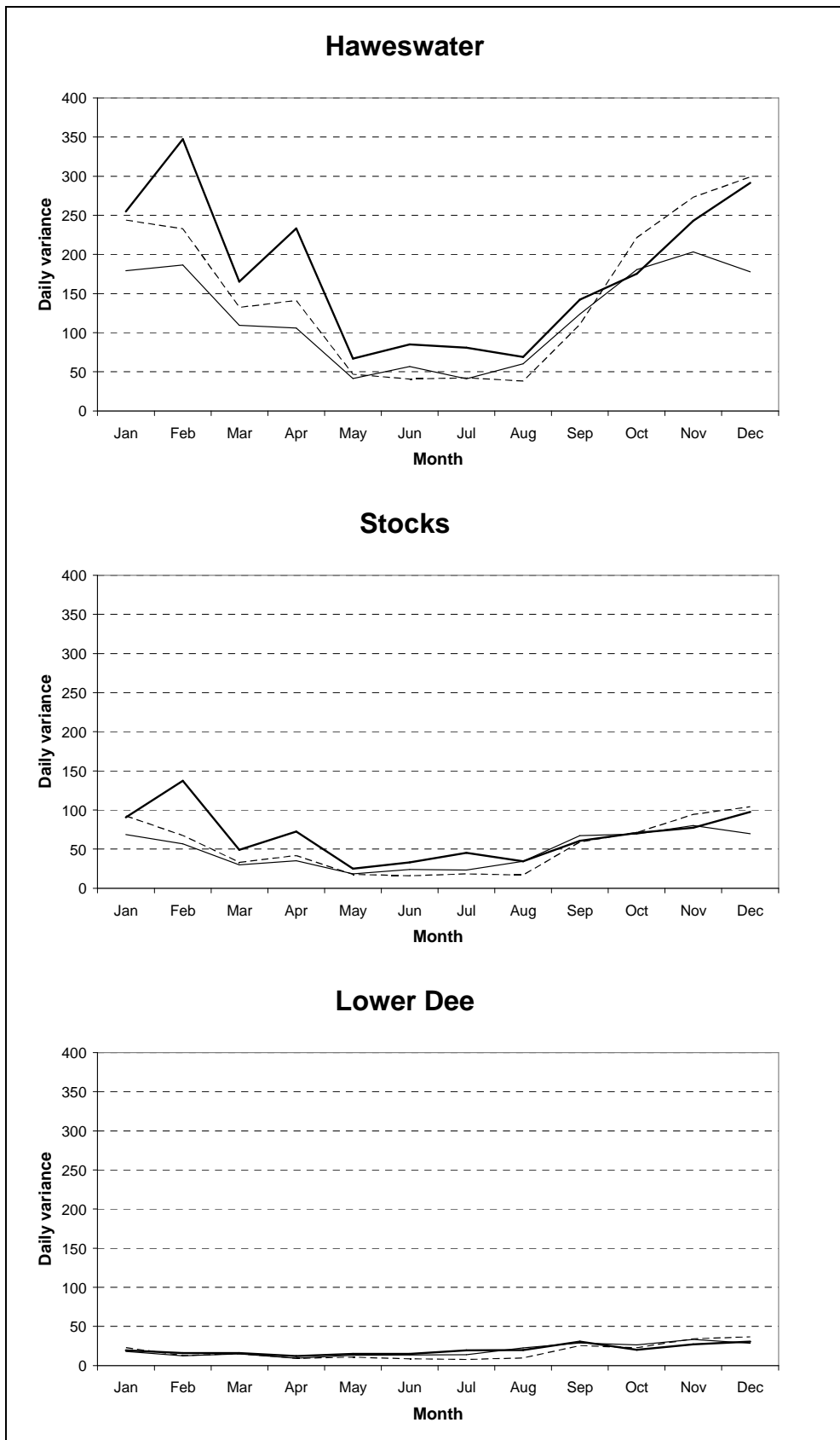
Figure 6 Comparison of daily variance for observed rainfall data (bold line), bias-corrected HadRM3H control scenario (line) and bias-corrected HadRM3H future scenario (dashed line).
