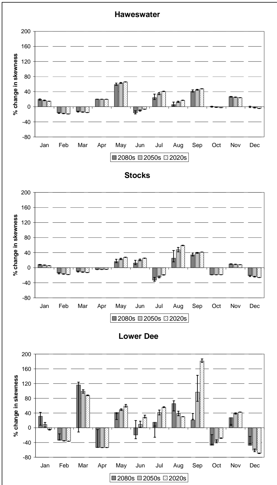
Figure 10 Percentage change in daily streamflow skewness between the HadRM3H control and future scenarios for the 2020s, 2050s and 2080s time-slices. Results shown are for the SRES A2 (UKCIP02 Medium-High) emissions scenario, but uncertainty bounds are given for the SRES A1 and B1 (UKCIP02 High and Low) emissions scenarios.
